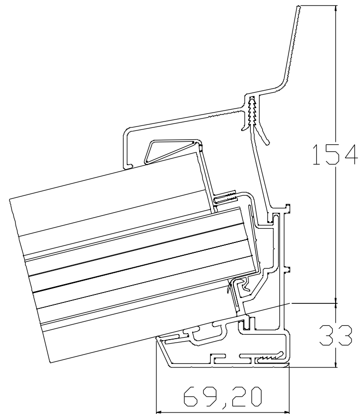
10 TO 15° MK2 VENTILATED WALLPLATE
